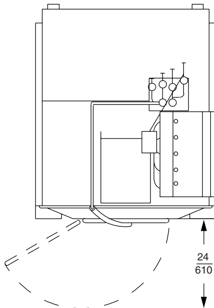
PLAN VIEW
