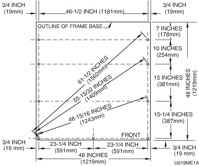
MOUNTING BOLT LAYOUT
