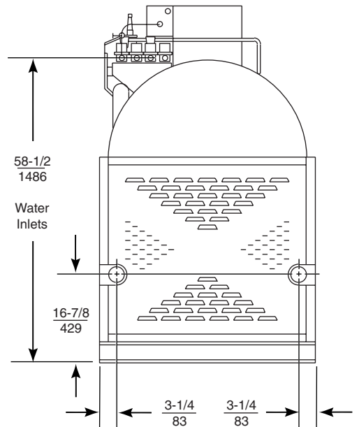
REAR VIEW
